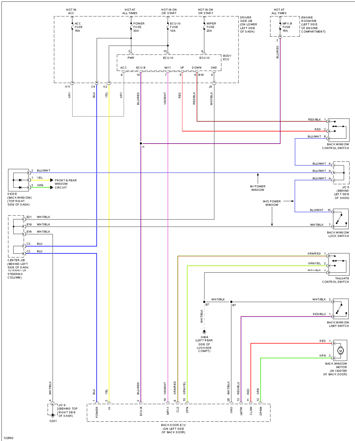
Fig. 42: Tailgate Power Window Circuit
