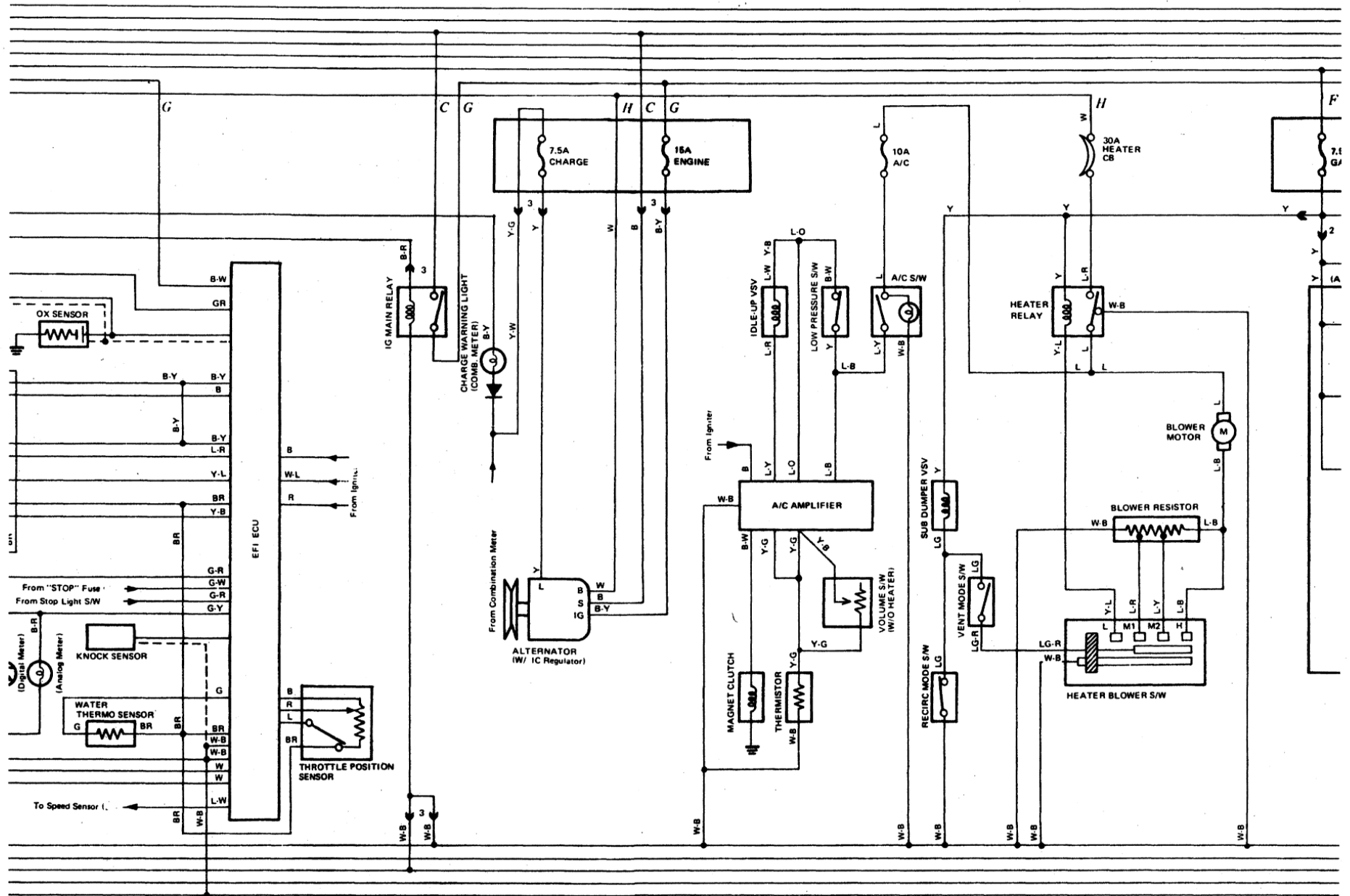
Typical 1982 and later model wiring diagram (2 of 9)
