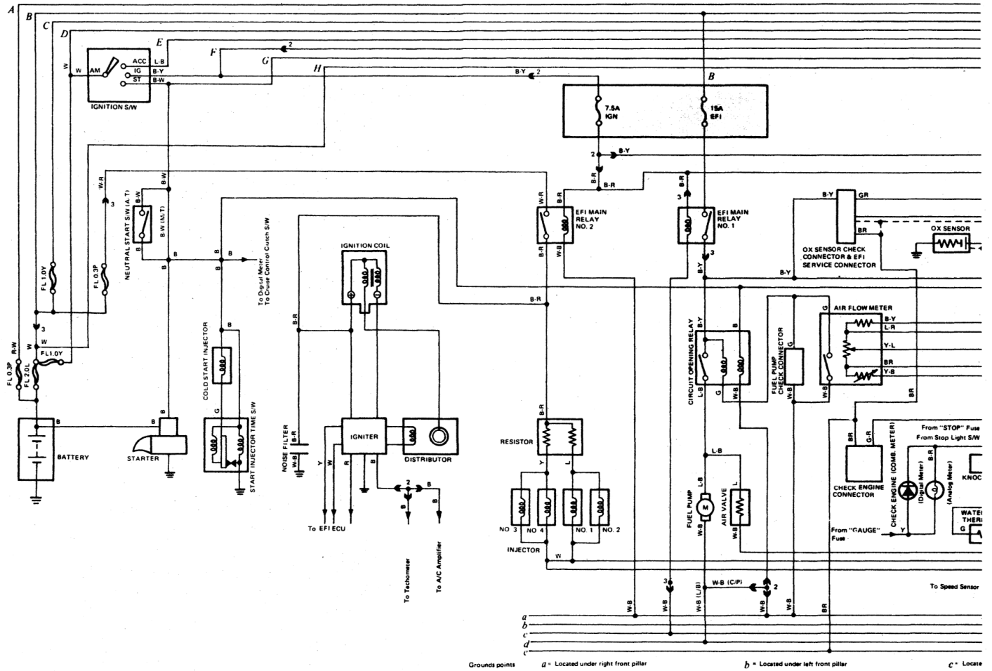
Typical 1982 and later model wiring diagram (1 of 9)
